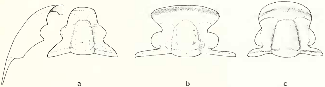
TEXT-FIG. 24. Dikelocephalinid cephalic structure and comparable forms. a , Proceratopyge (Upper Cambrian), showing form of cephalic doublure reflected in paradoublural line on prelabellar area. b , the dikelocephalinid Hungtioides (early Ordovician; after Fortey and Shergold 1984, pl. 44, fig. 2), showing similarity of paradoublural line to Proceratopyge , presumed to reflect similar course of doublure on venter. c , Chelidonocephalus (latest Middle Cambrian; after Wittke 1984, pl. 3), again showing similar prelabellar structure to a and b .
